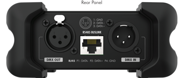
Rear Panel
